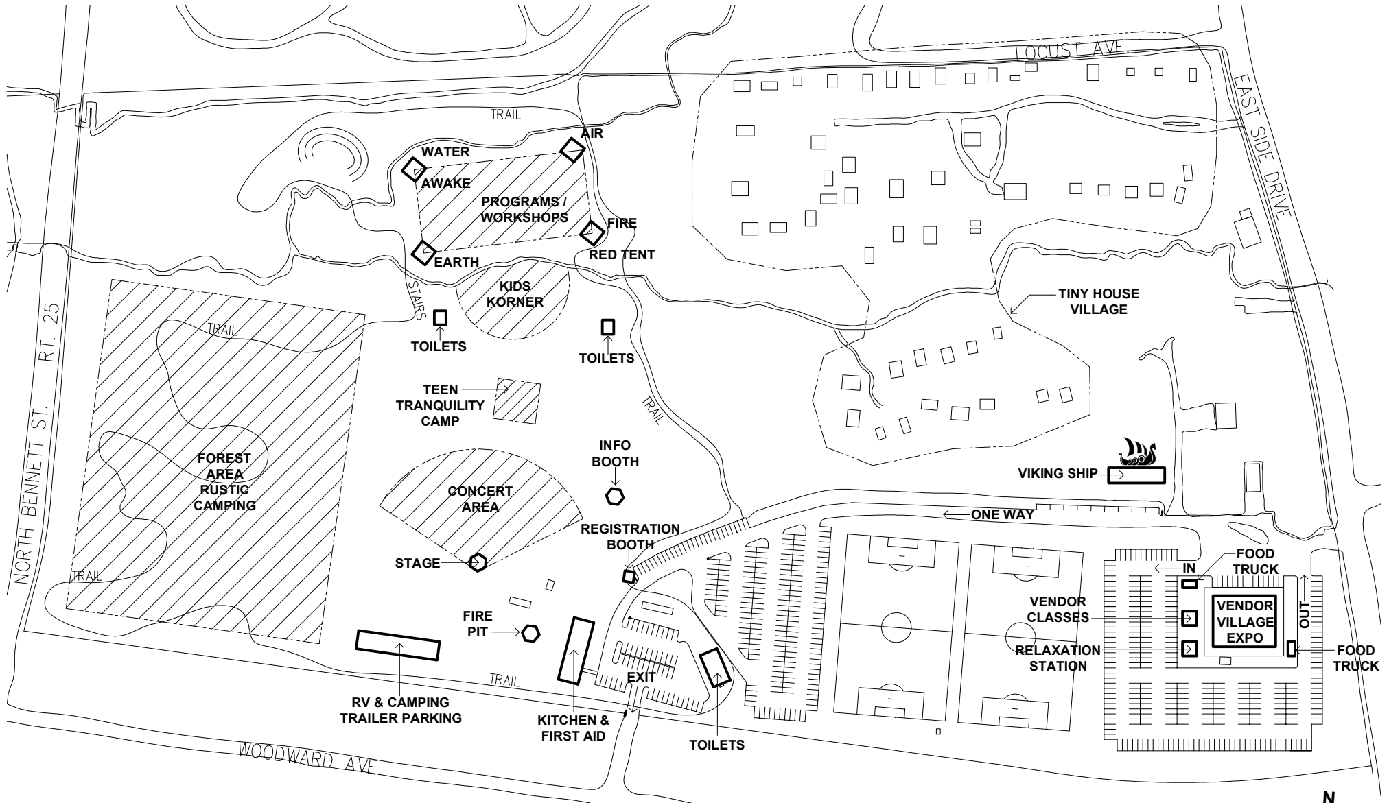
1 SITE PLAN
